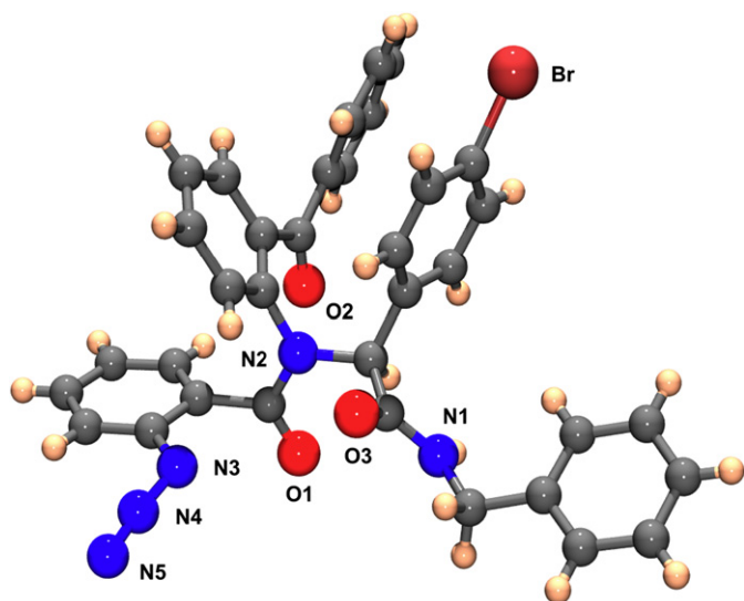
Figure 2. Single crystal X-ray diffraction structure of 5d .
