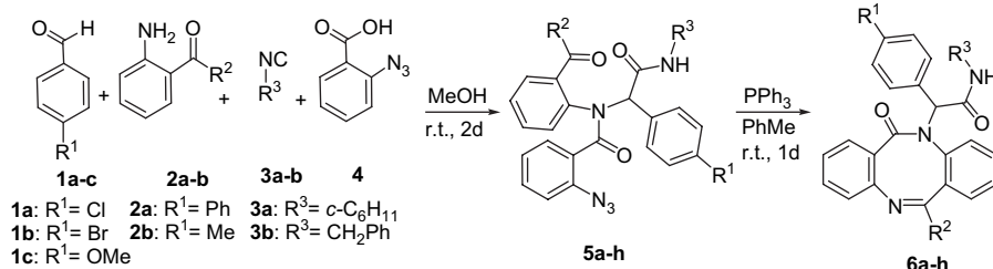
Scheme 1. Dibenzo[ b,f ][1,5]diazocine-5-yl arylglycinamides by the Ugi 4CC/Staudinger/aza-Wittig sequence.
